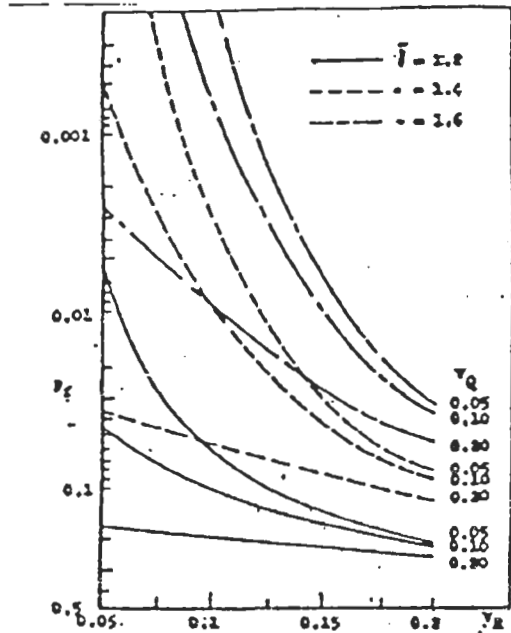
Figure 7. Probability of failure.
