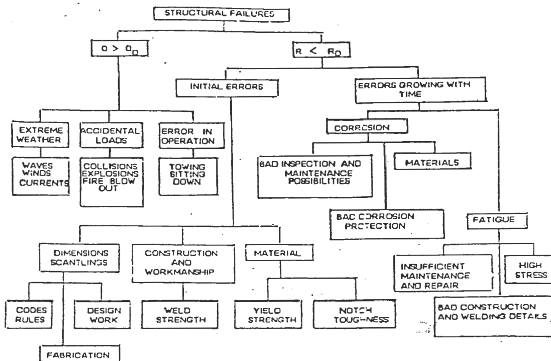
Figure 6. various causes of structural failure.
