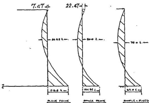
Figure 4. Effect of structural modelling.
